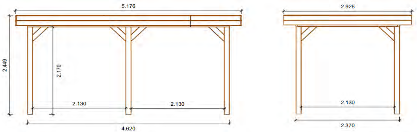
ALT23-1 500x300
